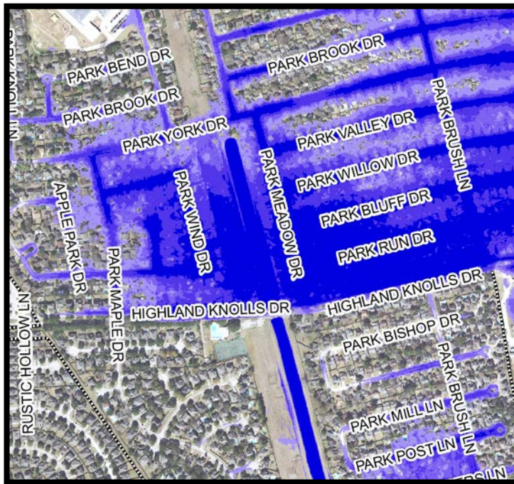
Existing 500-year Ponding
