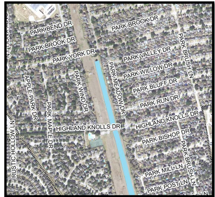
Proposed 500-year Ponding
